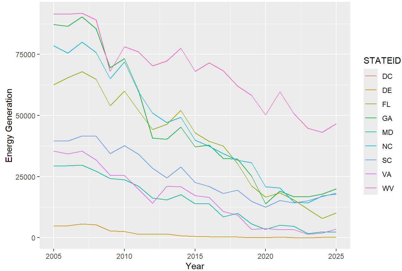
Coal Energy Generation by State (in thousand megawatthours)
