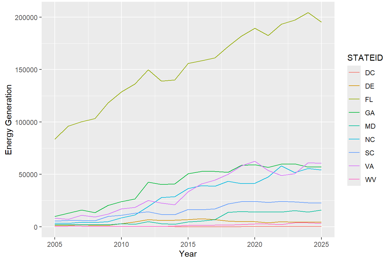
Natural Gas Energy Generation by State (in thousand megawatthours)
